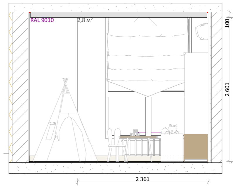
3-3 1:40
